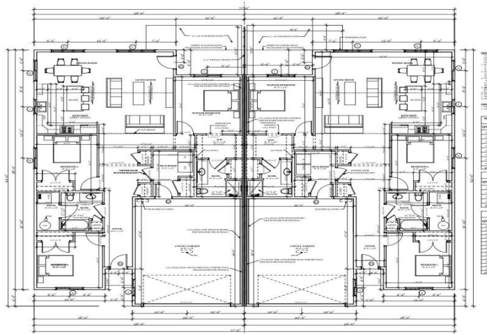
1 MAIN FLOOR PLAN SCALE: 1/4" = 1'-0"
