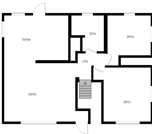
Upper Floor
