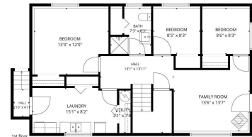
1st floor
