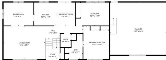
1st floor
