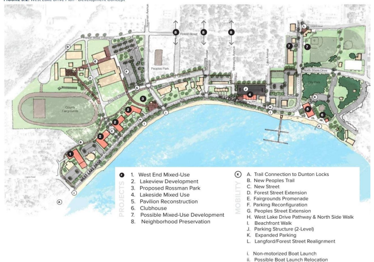
FIGURE 3.2. West Lake Drive Plan - Development Concept
