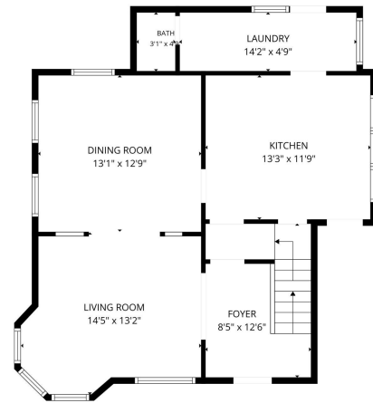
FLOOR PLAN CREATED BY CUBICSCANA APP. MEASUREMENTS DEEMED HIGHLY RELIABLE BUT NOT GUARANTEED.
