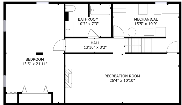
BASEMENT 1
