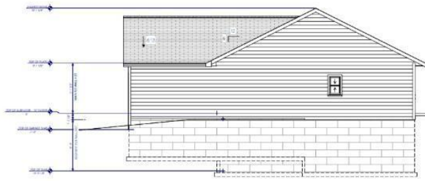
NORTH ELEVATION
